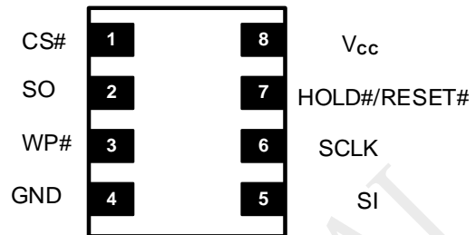
8-Land WSON (3x2mm)
