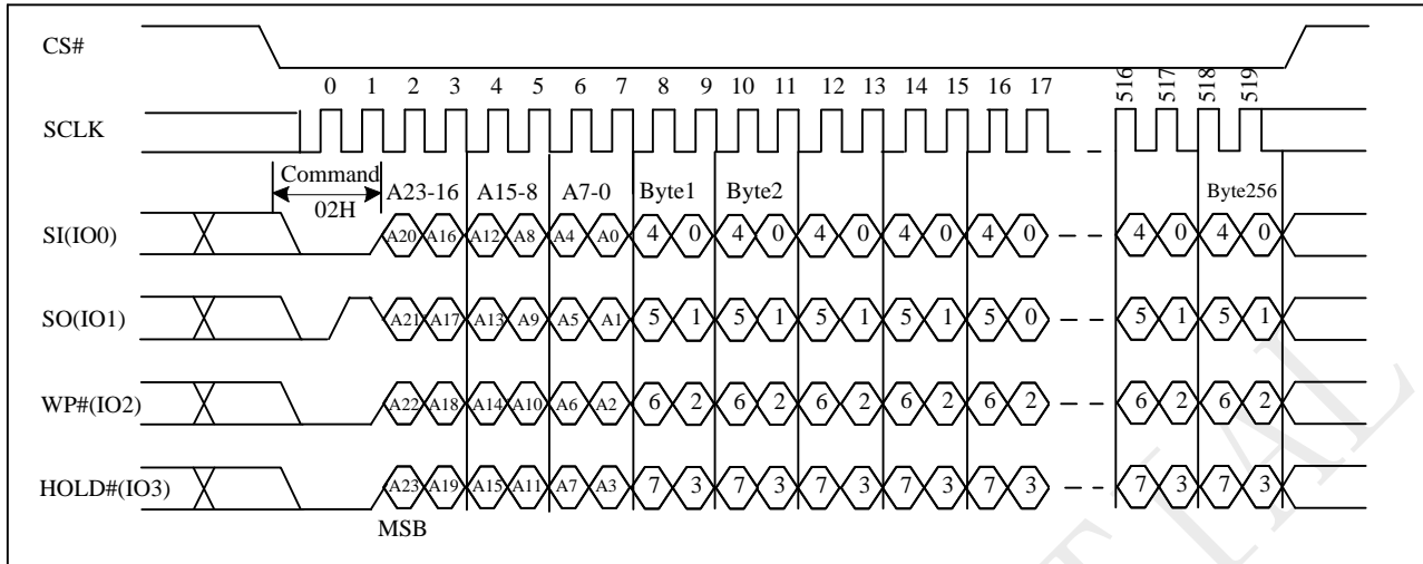
Figure 10-31a Page Program (PF) Sequence (QFI)
