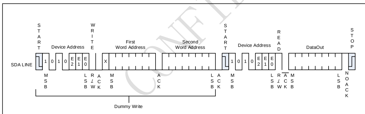
Figure 5-4 Random Read
