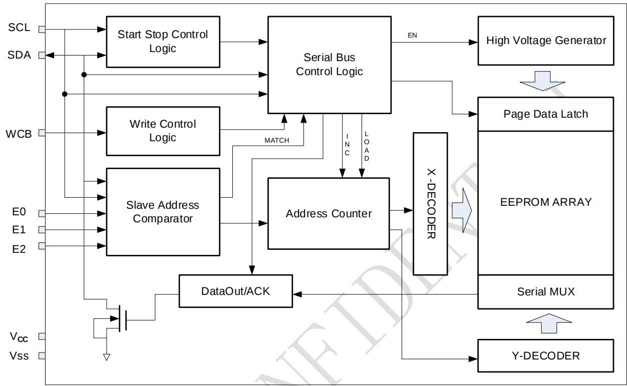
Figure 2-1 Block Diagram
